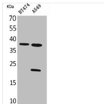
Western Blot analysis of BT474 A549 cells using IFN- \alpha 1 Polyclonal Antibody
