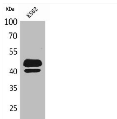
Western Blot analysis of K562 cells using PSG1 Polyclonal Antibody
