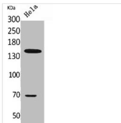
Western Blot analysis of HeLa cells using CD42b Polyclonal Antibody.
