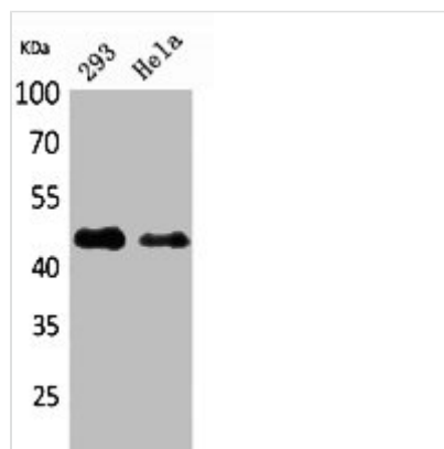
Western Blot analysis of 293, HeLa cells using IDH1 Polyclonal Antibody.
