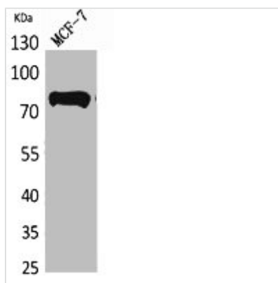
Western Blot analysis of MCF7 cells using c-Myb Polyclonal Antibody.
