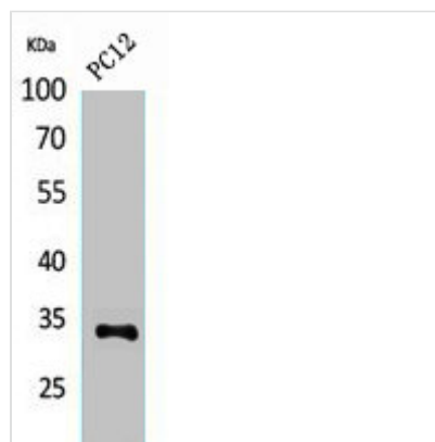
Western Blot analysis of PC12 cells using CD74 Polyclonal Antibody.
