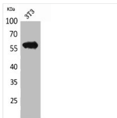
Western Blot analysis of NIH-3T3 cells using CD223 Polyclonal Antibody.
