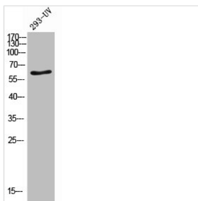
Western Blot analysis of 293-UV cells using CD96 Polyclonal Antibody
