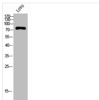
Western Blot analysis of LOVO cells using Calpain 10 Polyclonal Antibody
