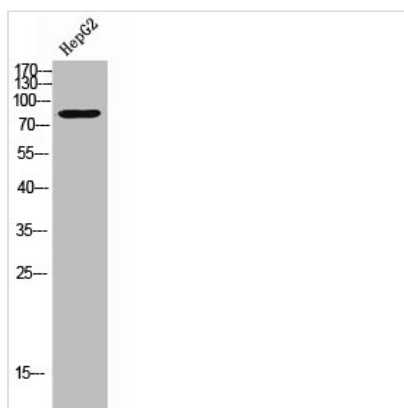
Western Blot analysis of HepG2 cells using CNG-1 Polyclonal Antibody
