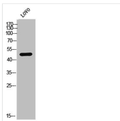
Western Blot analysis of LOVO cells using Casein Kinase Iε Polyclonal Antibody
