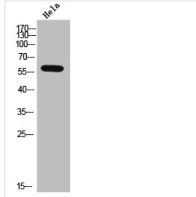
Western Blot analysis of HELA cells using ALS2CR13 Polyclonal Antibody
