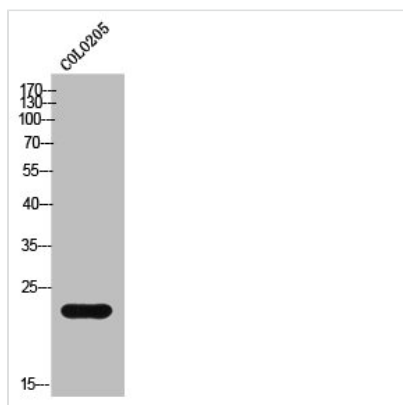
Western Blot analysis of COLO205 cells using Cathepsin G Polyclonal Antibody
