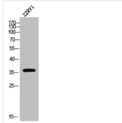
Western Blot analysis of 22RV1 cells using AR-β3 Polyclonal Antibody
