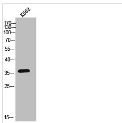
Western Blot analysis of K562 cells using AR-β3 Polyclonal Antibody
