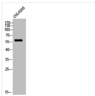
Western Blot analysis of COLO205 cells using Elongin A3 Polyclonal Antibody
