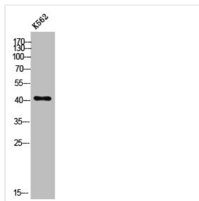
Western Blot analysis of K562 cells using ZnT-8 Polyclonal Antibody
