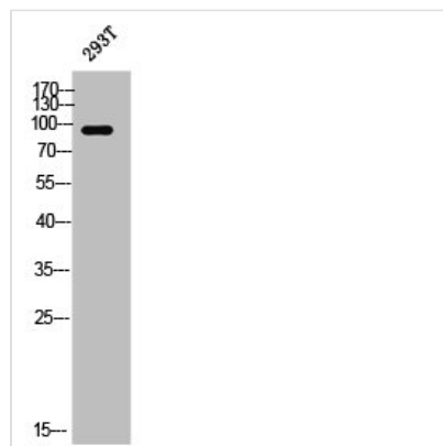
Western Blot analysis of 293T cells using PSD-95 Polyclonal Antibody
