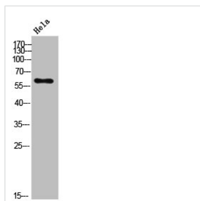
Western Blot analysis of HeLa cells using Phospho-CRMP-2 (S522) Polyclonal Antibody
