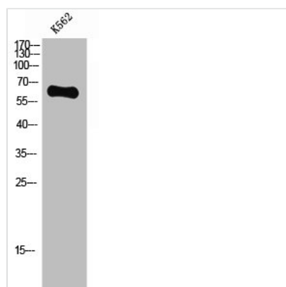
Western Blot analysis of K562 cells using Glypican-5 Polyclonal Antibody
