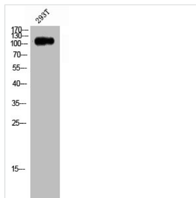
Western Blot analysis of 293T cells using CNK2 Polyclonal Antibody
