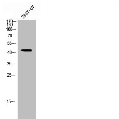
Western Blot analysis of 293 cells using SIRT2 Polyclonal Antibody
