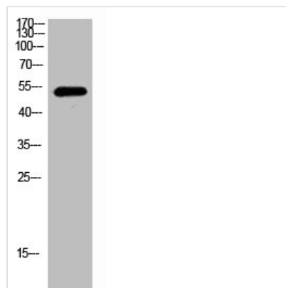
Western Blot analysis of mouse cells using NDR2 Polyclonal Antibody
