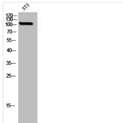
Western Blot analysis of 3T3 cells using GluR- \delta 2 Polyclonal Antibody
