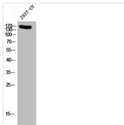
Western Blot analysis of 293T-UV cells using Phospho-NMDAε2 (Y1336) Polyclonal Antibody
