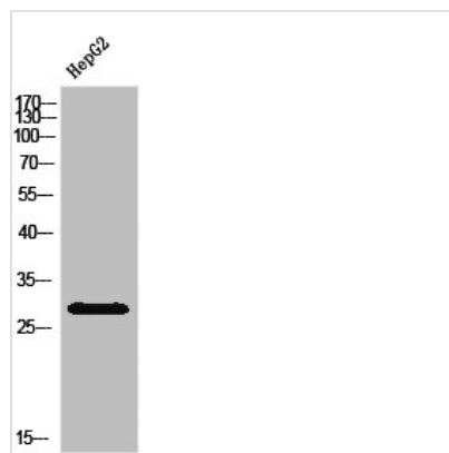
Western Blot analysis of HepG2 cells using IGFBP1 Polyclonal Antibody
