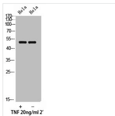
Western Blot analysis of HELA cells using Phospho-Smad3 (T179) Polyclonal Antibody
