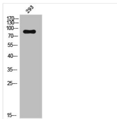
Western Blot analysis of 293 cells using Phospho-CD71 (S24) Polyclonal Antibody
