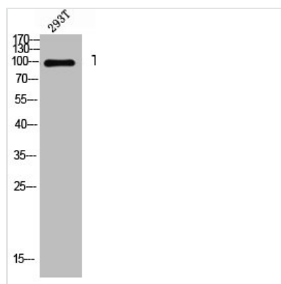
Western blot analysis of 293T lysis using Thrombospondin 4 antibody.
