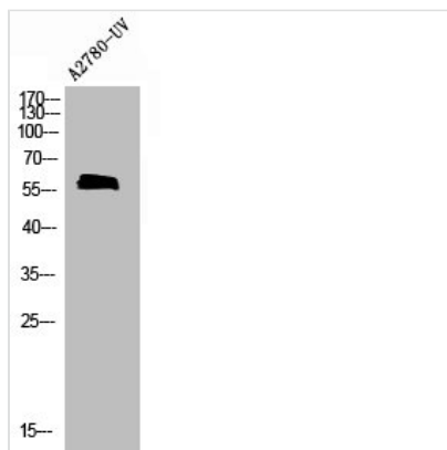
Western Blot analysis of Jurkat cells using Phospho-Cdc25A (S75) Polyclonal Antibody
