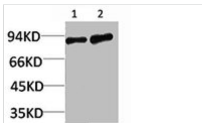
Western blot analysis of 1) Mouse Brain, 2) Rat Brain using HIF-1 \beta Polyclonal Antibody.
