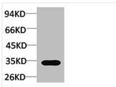
Western blot analysis of Hela using Caspase-3 Polyclonal Antibody.
