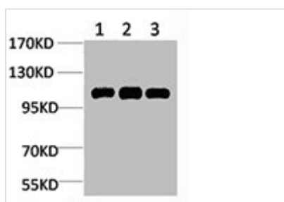
Western blot analysis of 1) 3T3, 2) PC12, 3) Rat Heart Tissue using Actinin- \alpha 1 Polyclonal Antibody.
