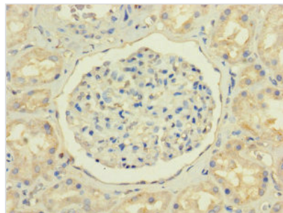
Immunohistochemistry of paraffin-embedded human kidney tissue using CSB-PA015976LA01HU at dilution of 1:100
