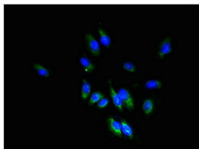
Immunofluorescent analysis of HeLa cells using CSB-PA025146LA01HU at dilution of 1:100 and Alexa Fluor 488-conjugated AffiniPure Goat Anti-Rabbit IgG(H+L)
