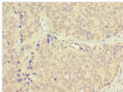
Immunohistochemistry of paraffin-embedded human gastric cancer using CSB-PA842631LA01HU at dilution of 1:100
