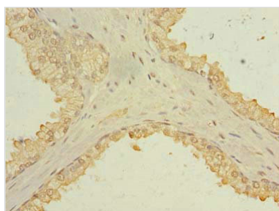
Immunohistochemistry of paraffin-embedded human prostate cancer using CSB-PA842631LA01HU at dilution of 1:100
