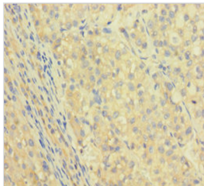
Immunohistochemistry of paraffin-embedded human liver cancer using CSB-PA011156LA01HU at dilution of 1:100
