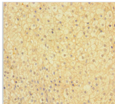
Immunohistochemistry of paraffin-embedded human adrenal gland tissue using CSB-PA880093LA01HU at dilution of 1:100
