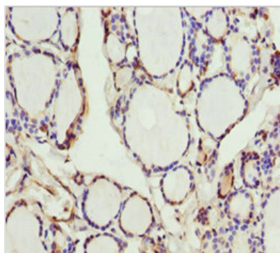
Immunohistochemistry of paraffin-embedded human thyroid tissue using CSB-PA856936ESR2HU at dilution of 1:100
