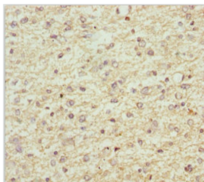
Immunohistochemistry of paraffin-embedded human glioma using CSB-PA856936ESR2HU at dilution of 1:100
