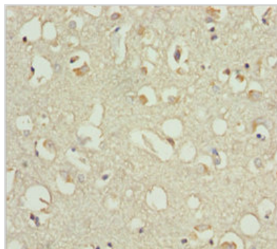
Immunohistochemistry of paraffin-embedded human brain tissue using CSB-PA335050DSR2HU at dilution of 1:100
