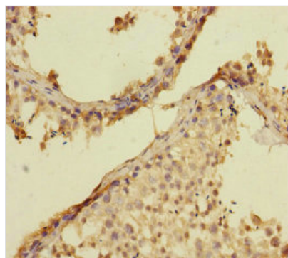
Immunohistochemistry of paraffin-embedded human testis tissue using CSB-PA019178ESR2HU at dilution of 1:100
