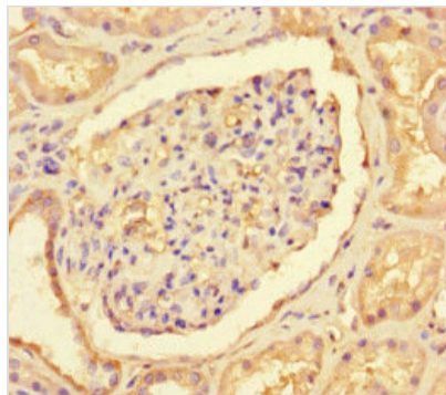
Immunohistochemistry of paraffin-embedded human kidney tissue using CSB-PA005663LA01HU at dilution of 1:100
