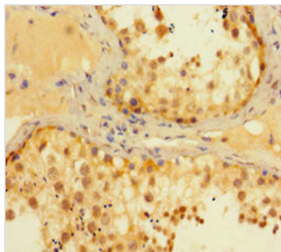
Immunohistochemistry of paraffin-embedded human testis tissue using CSB-PA013694HA01HU at dilution of 1:100
