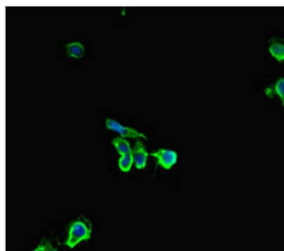
Immunofluorescent analysis of HeLa cells using CSB-PA880936LA01HU at dilution of 1:100 and Alexa Fluor 488-conjugated AffiniPure Goat Anti-Rabbit IgG(H+L)
