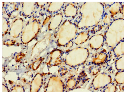
Immunohistochemistry of paraffin-embedded human thyroid tissue using CSB-PA880936LA01HU at dilution of 1:100
