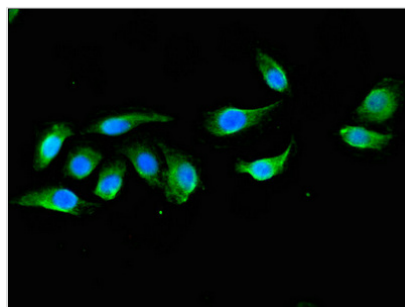
Immunofluorescent analysis of A549 cells using CSB-PA007019LA01HU at dilution of 1:100 and Alexa Fluor 488-conjugated AffiniPure Goat Anti-Rabbit IgG(H+L)
