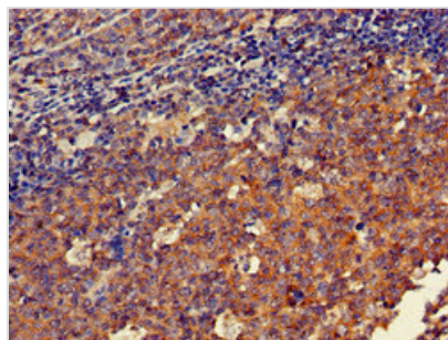
Immunohistochemistry of paraffin-embedded human tonsil tissue using CSB-PA007019LA01HU at dilution of 1:100
