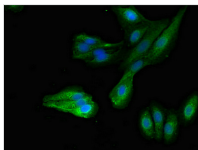
Immunofluorescent analysis of HepG2 cells using CSB-PA839876LA01HU at dilution of 1:100 and Alexa Fluor 488-conjugated AffiniPure Goat Anti-Rabbit IgG(H+L)
