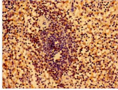
Immunohistochemistry of paraffin-embedded human spleen tissue using CSB-PA642773LA01HU at dilution of 1:100
