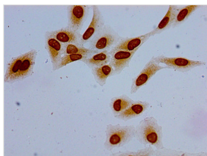
Immunocytochemistry analysis of HeLa cells using CSB-PA010380PA63acHU at dilution of 1:100
