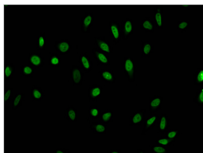
Immunofluorescent analysis of HeLa cells (sodium butyrate, 30 mM, 4h) using CSB-PA010380PA63acHU at dilution of 1:100 and Alexa Fluor 488-conjugated AffiniPure Goat Anti-Rabbit IgG(H+L)
