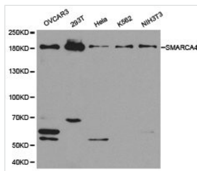
Western blot analysis of extracts of various cell lines, using SMARCA4 antibody.
