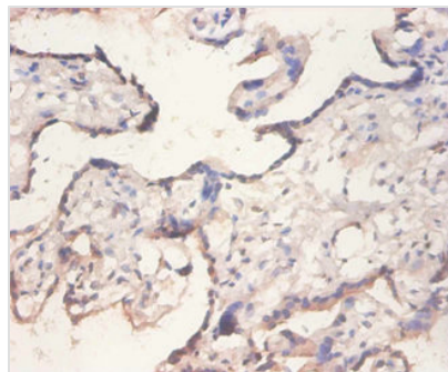
Immunohistochemistry of paraffin-embedded human placenta tissue using CSB-PA007563DA01HU at dilution of 1:100
